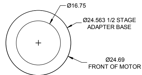
FRONT VIEW (WITH FIN REMOVED)
